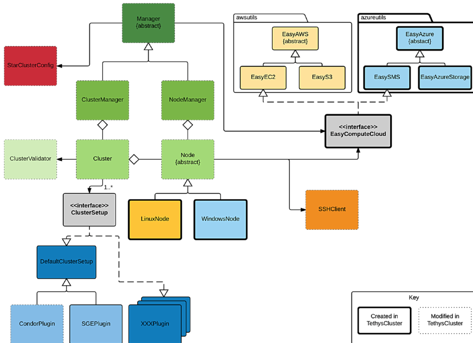
Figure 3-4. UML diagram showing classes that I modified and the classes and modules that I added in TethysCluster.
